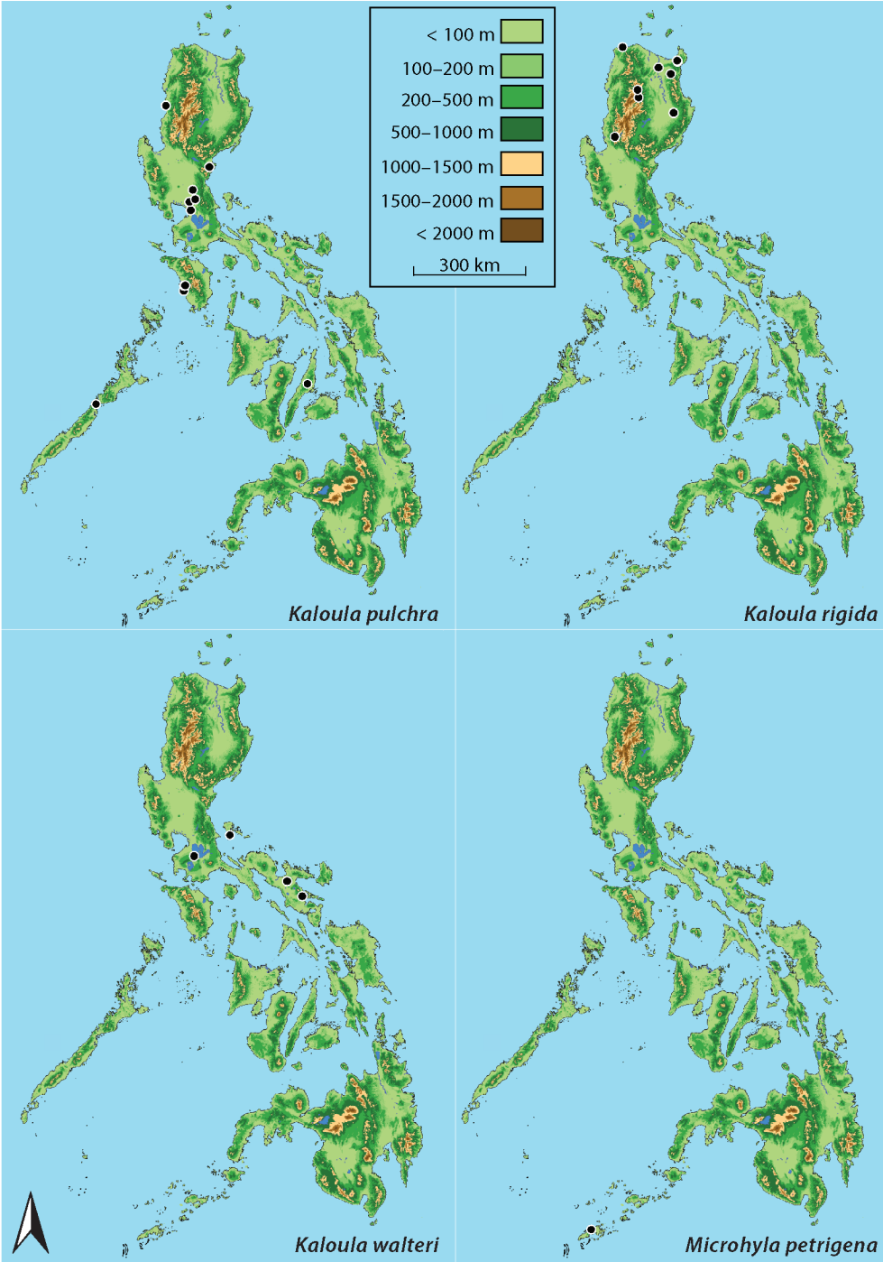
FIGURE 20. Geographic range maps for members of the family Microhylidae ( Kaloula pulchra , K. rigida , K. waltheri , and Microhyla petrigena ). Points represent museum vouchered specimens with georeferenced locality information overlaid on a topographic map of the Philippines.
